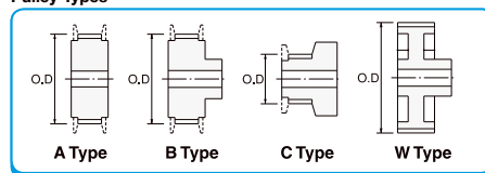
Pulley Types
